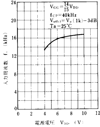
f_i - V_{DD}
