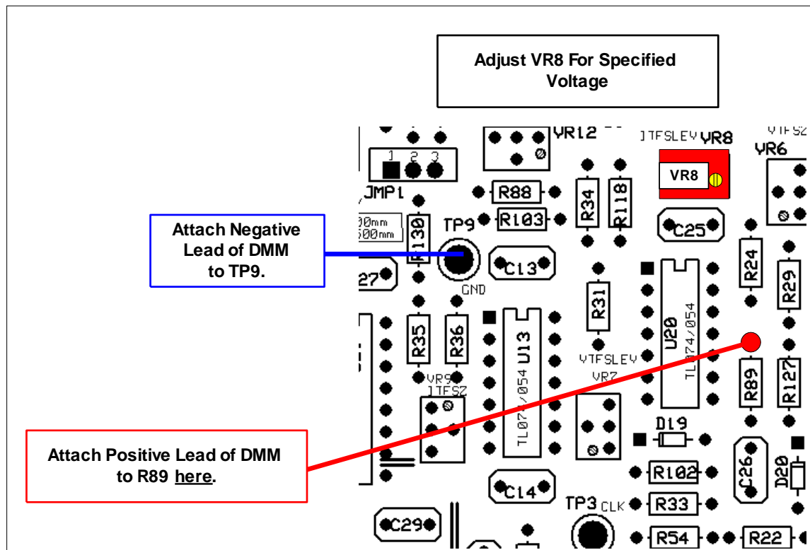
Figure 9-14: Initial Current TFS Range Calibration
