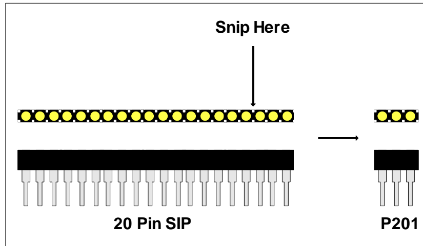
Figure 7-4: Creating P201 from a 20 Pin SIP
