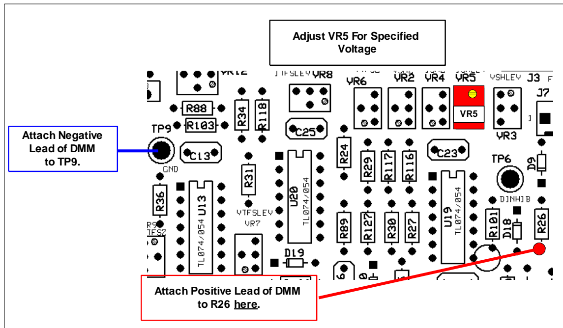
Figure 9-11: Initial Range Voltage Calibration
