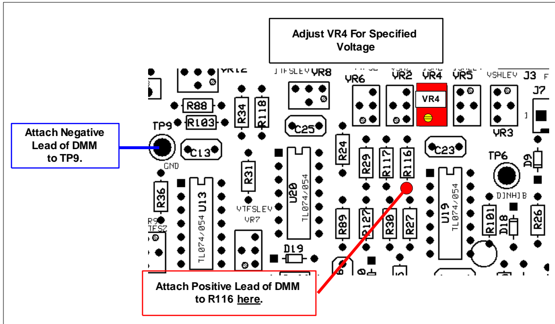
Figure 9-10: Initial Zero Voltage Calibration
