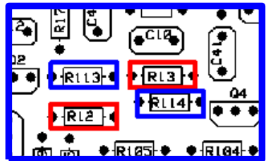
Figure 8-11: Gate/Trigger Level Resistor Locations
