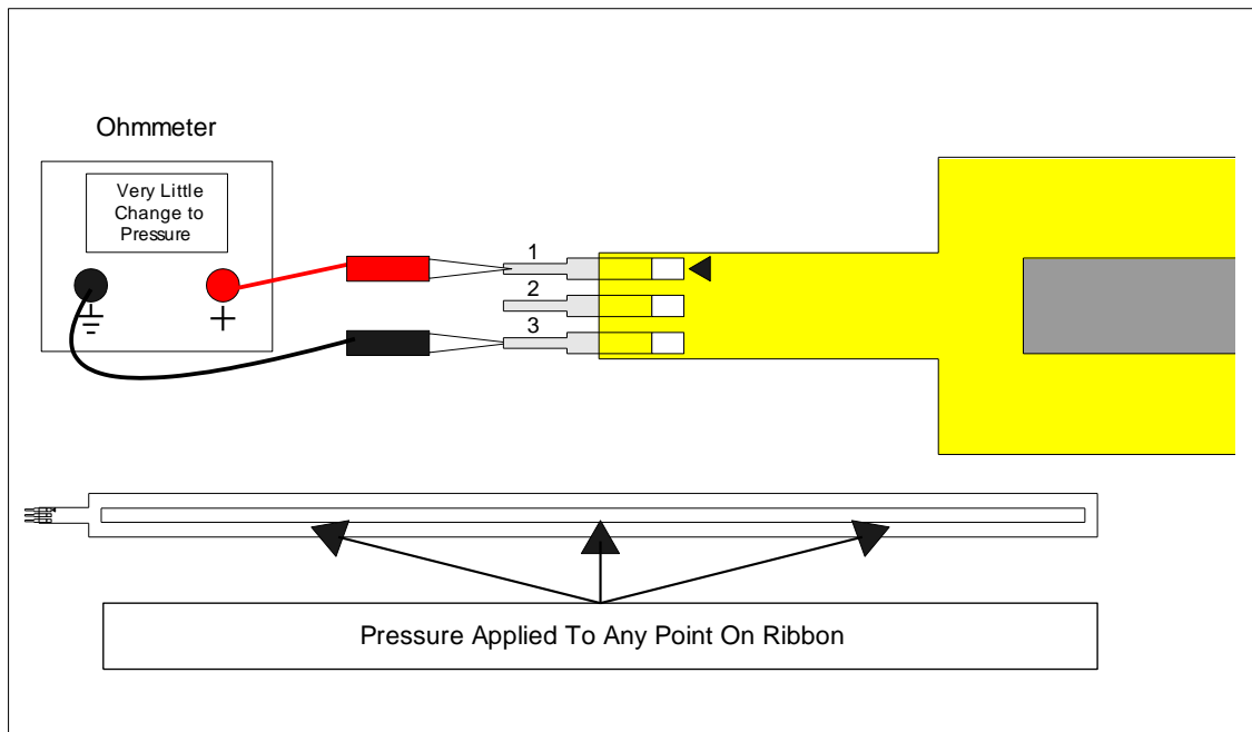
Figure 7-3: Testing the “Outside” Pins of the SoftPot®
