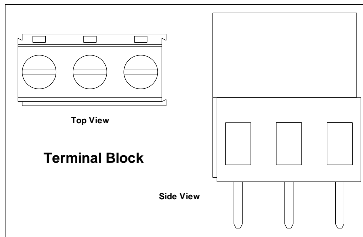
Figure 8-3A: Depiction of a Terminal Block Connector, Tyco® Part No. 796949-3
