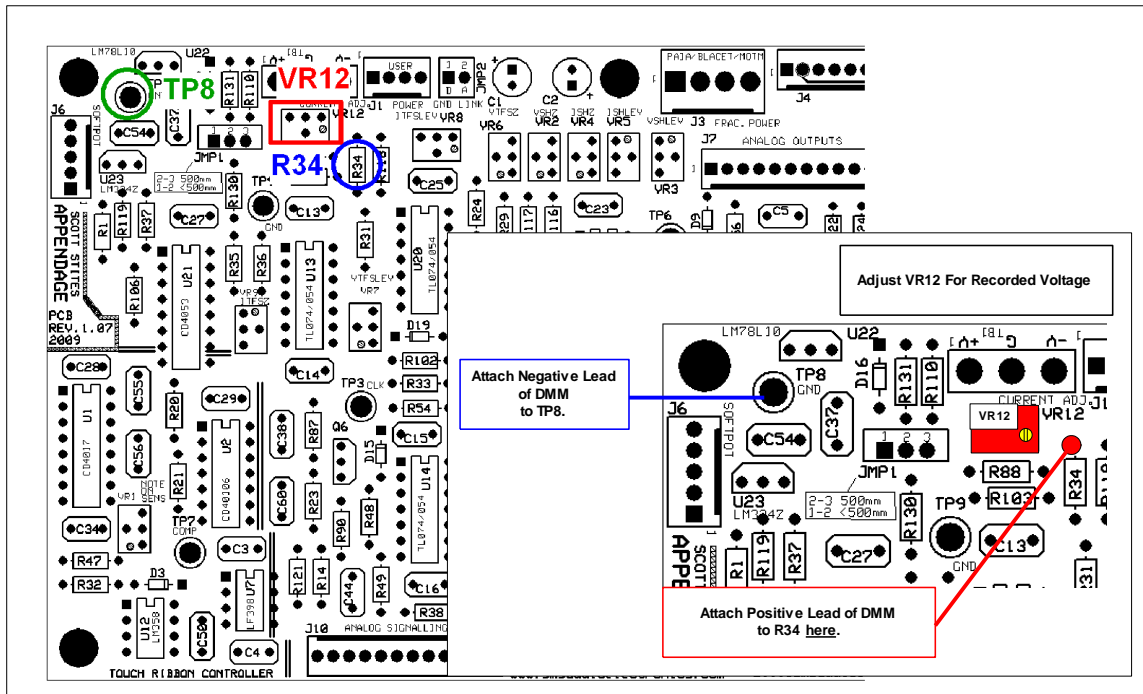
Figure 9-1: Ribbon Current Calibration Points
