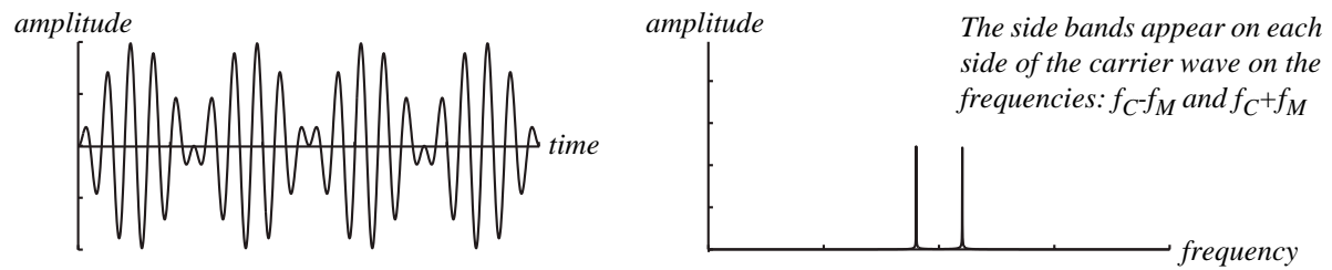
Fig 3. Ring Modulation
