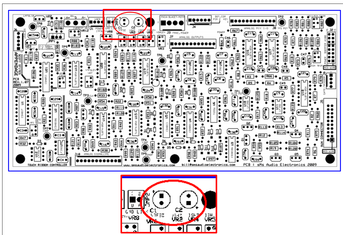
Figure 8-32: Locations for C1, C2
