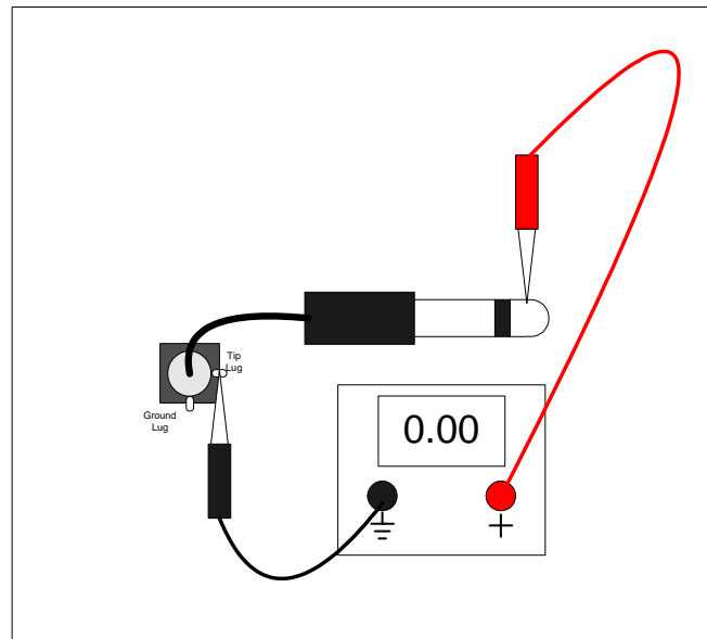
Figure 3-11: Locating the Tip Lug
