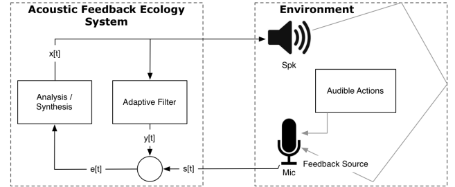
Figure 4: The Block diagram of AFES.
